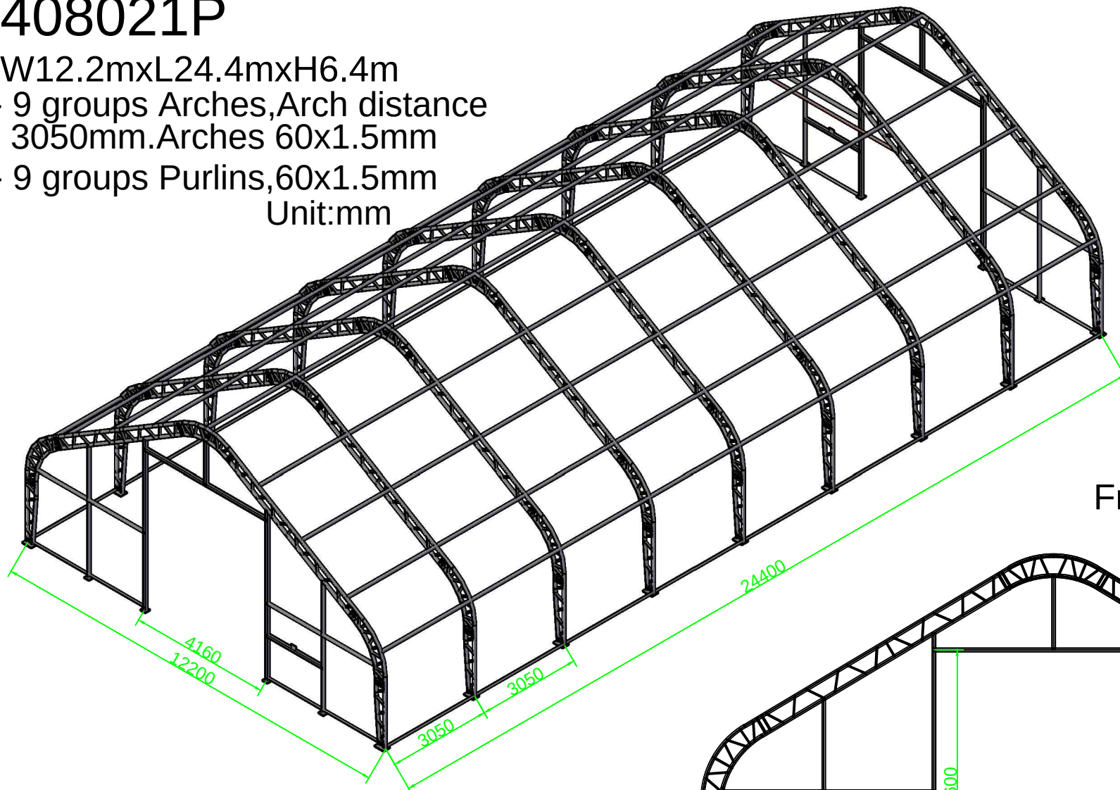
Frame Sketch
